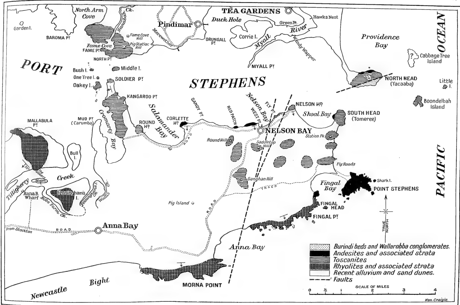
Geological Map, Port Stephens District.
